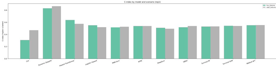
Fig. 1 C-index by model, four_features vs. eight_features (rep1).
